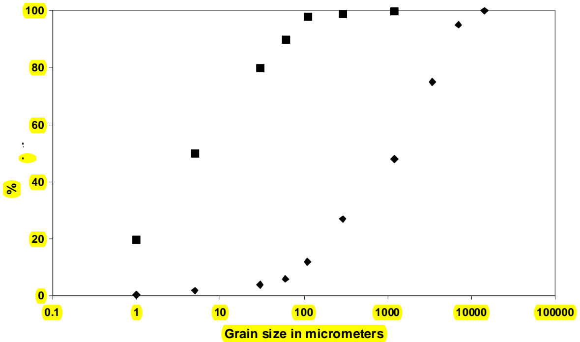
Cumulative distribution of grain size for fly and bottom ash
